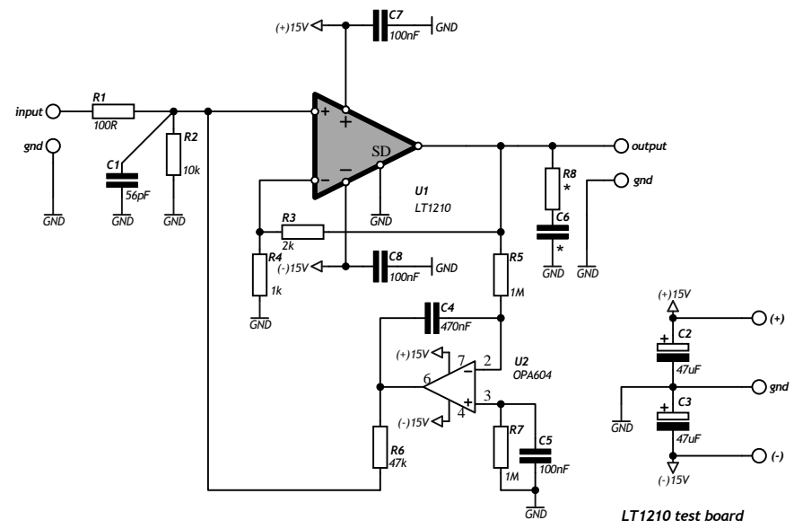
LT1210 test board
