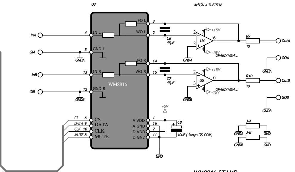
WM8816 STAMP Stereo volume control Damian Antoniak antoniak@unisonus.com
